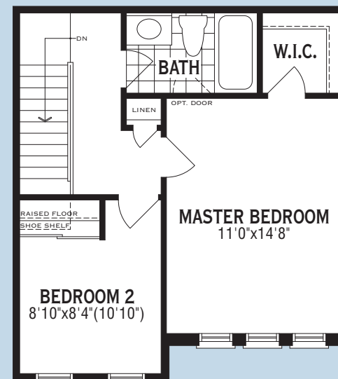
Third Floor Plan 2 Bedroom
